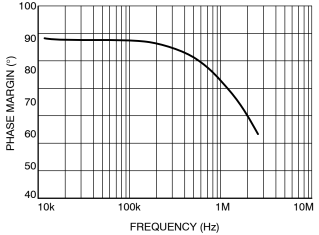
Figure 4. Open Loop Phase Margin ( R_L = 2\text{ k}\Omega , T_A = 25^\circ\text{C} )
