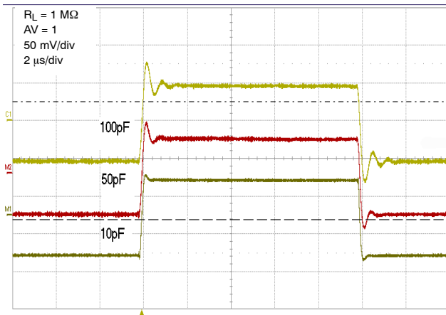
Figure 23. Settling Time vs. Capacitive Load
